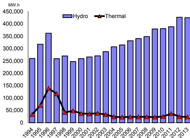
Hydro and Thermal Generation, Yukon, 1994 to 2013
